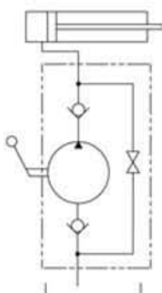
Inline schematic
