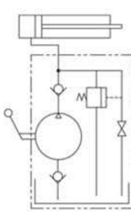
S/A with relief schematic
