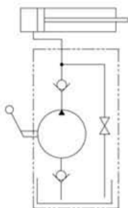
S/A schematic
