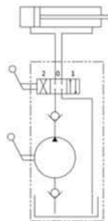
D/A schematic
